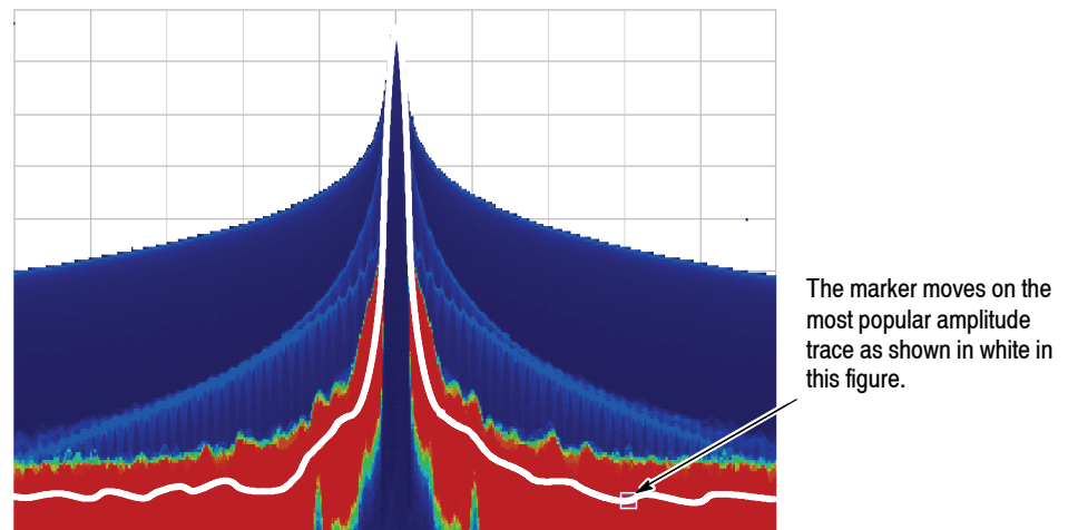
Figure 3- 158: Marker movement on the Bitmap trace
