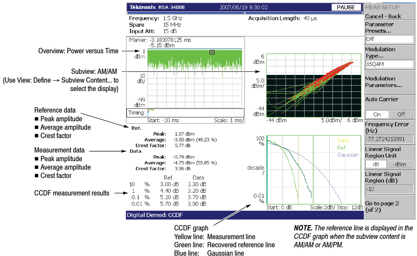
Figure 3-51: CCDF measurement
