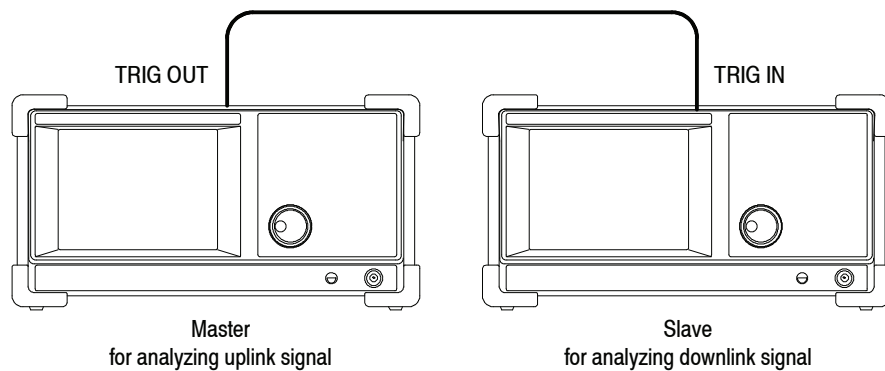
Figure 3- 116: Synchronous operation of two RSA3408B analyzers
