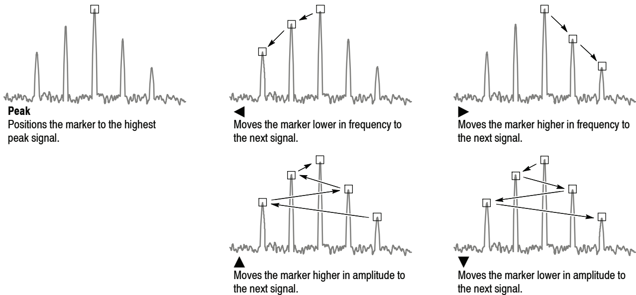
Figure 3-159: Functions of the peak search keys
