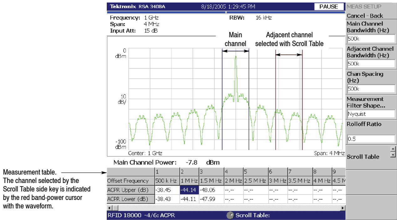
Figure 3-56: ACPR measurements
