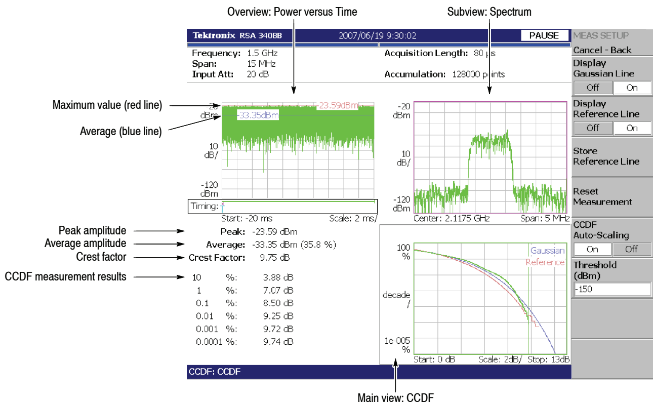
Figure 3-70: CCDF multi-view
