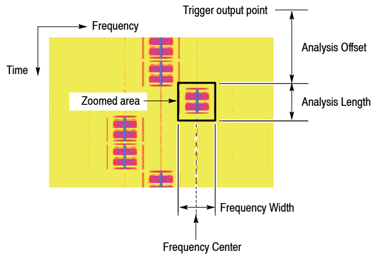
Figure 3-25: Zoom domain settings using the acquisition and analysis menu
