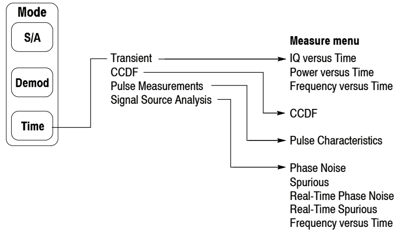
Figure 3-64: Time menu structure
