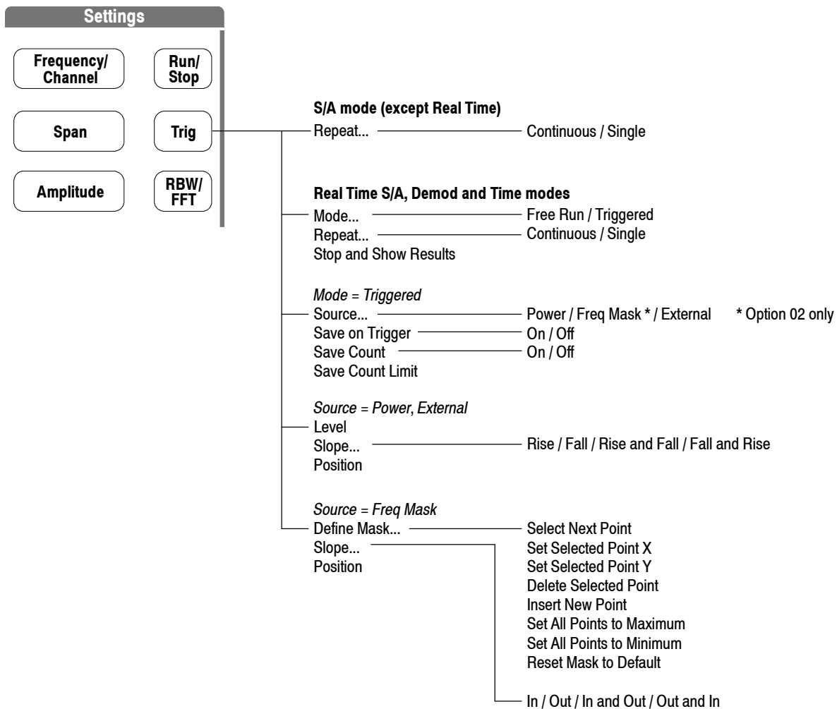
Figure 3- 103: Trigger menu structure
