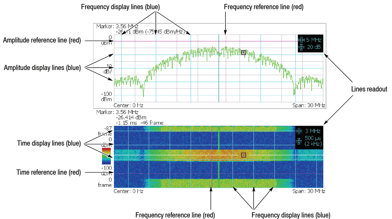
Figure 3-149: Multi display lines (Real Time S/A mode)
