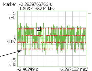
Figure 3-44: IQ/Frequency versus time measurement
