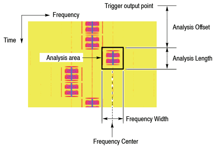
Figure 3- 100: Parameters in the zoom mode
