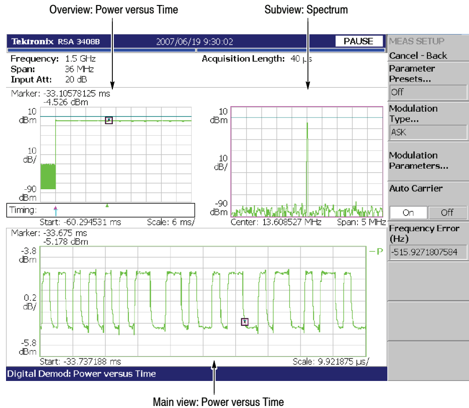
Figure 3-45: Power variance measurement
