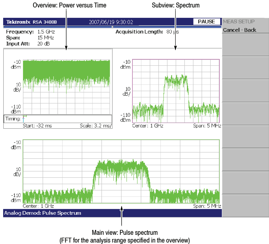
Figure 3-40: Pulse spectrum measurement
