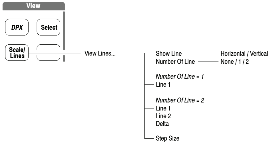
Figure 3- 146: Lines menu structure (other than Real Time S/A)
