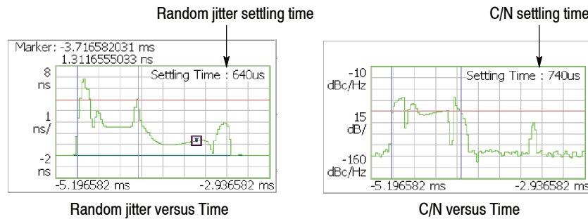
Figure 3-81: Settling time displayed in the subview
