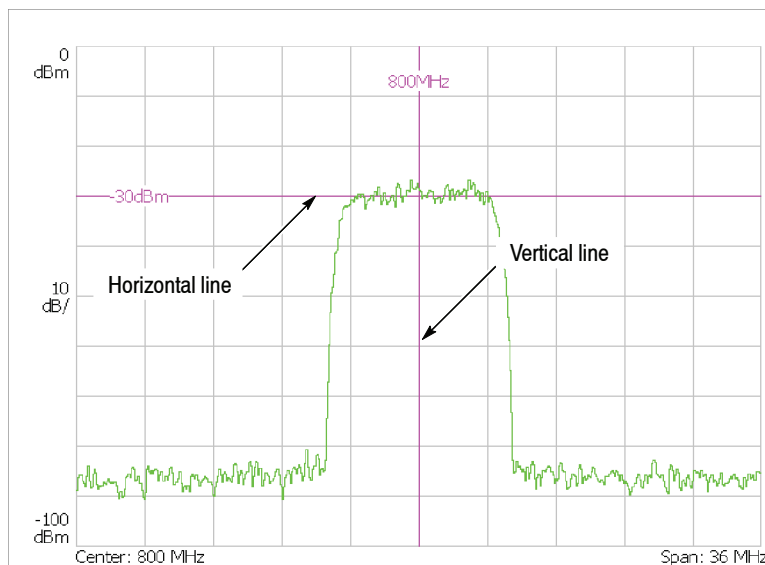
Figure 3-145: Display line
