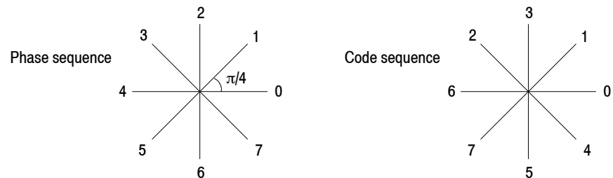
Figure 3- 139: D8PSK symbol value
